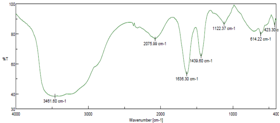
Graph 2: FTIR Analysis for skin Extract
