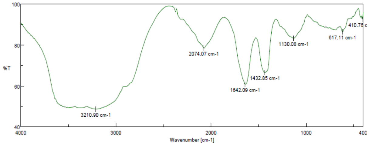
Graph 1: FTIR Analysis for tissue extract
