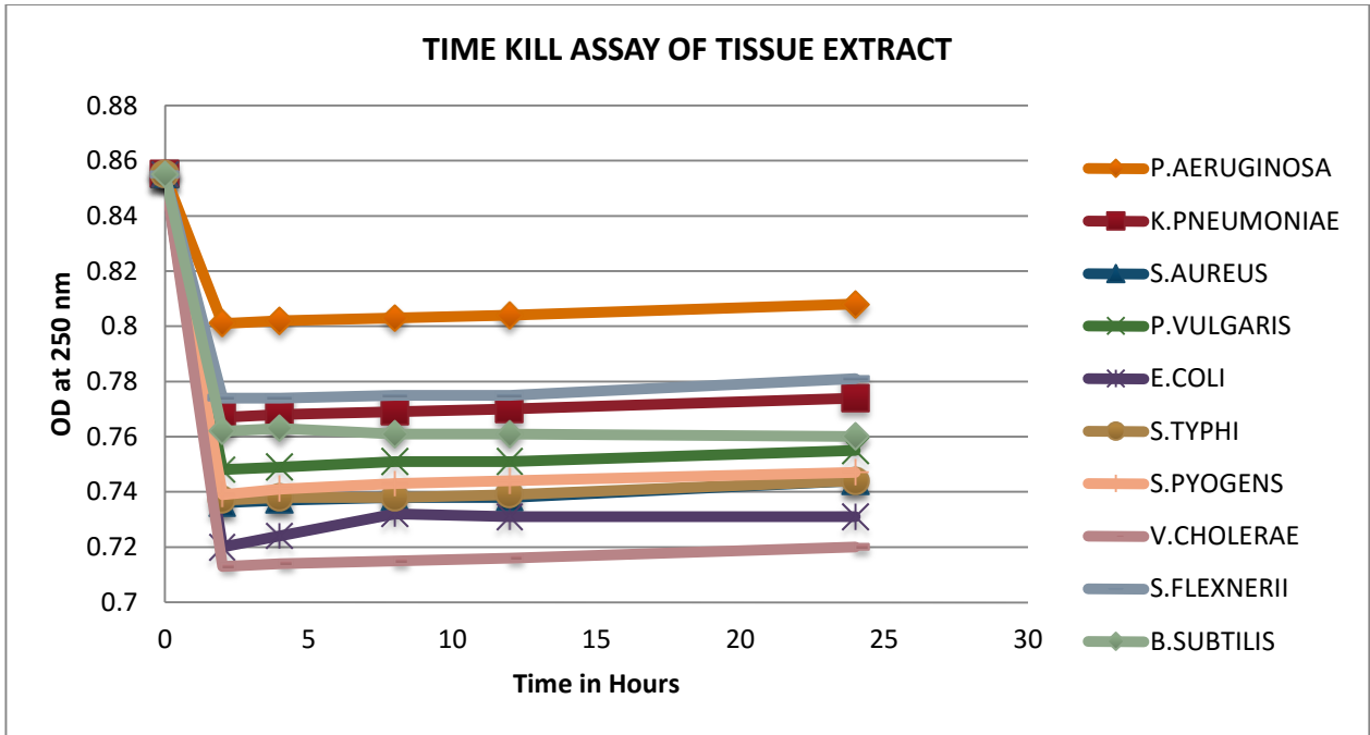
Graph 3: Time kill kinetics of tissue extract
