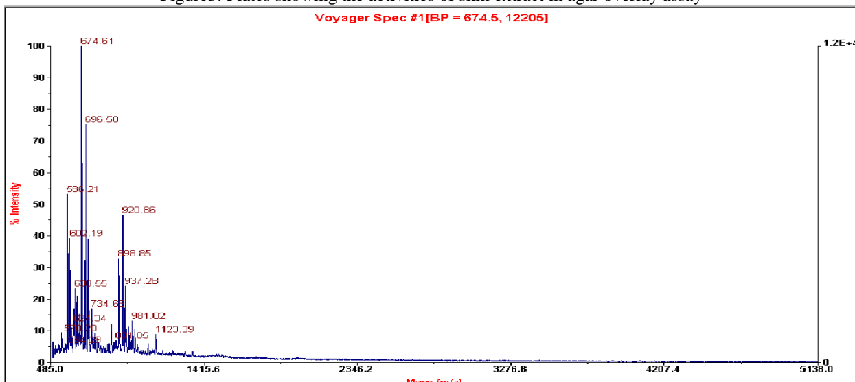
Graph 7: Mass Spectrum of Tissue Fraction
