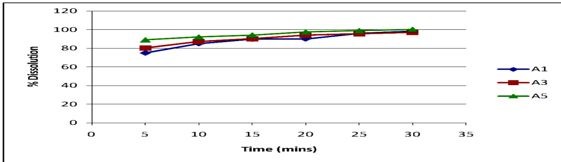
Figure 6: Dissolution profile of formulations A 1 , A 3 and A 5
