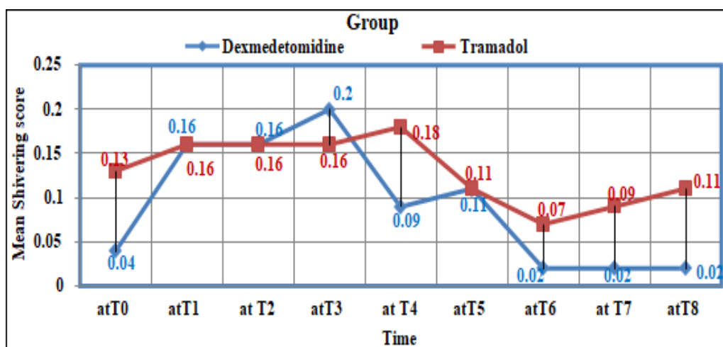
Figure1: Distribution of shivering score at various time intervals in both the groups.
