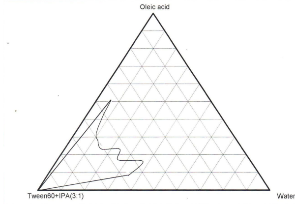
Figure 3: Pseudoternary phase diagram for microemulsion using oleic acid, tween 60+IPA (3:1) & water
