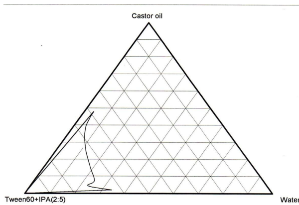
Figure 5: Pseudoternary phase diagram for microemulsion system, using castor, Tween 60+IPA (2:5) & water
