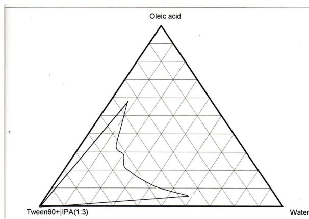
Figure 1: Pseudoternary phase diagram for microemulsion using Oleic acid, Tween60+IPA (1:3) & water
