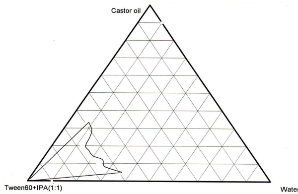
Figure 4: Pseudoternary phase diagram for microemulsion system, using castor oil, Tween 60+IPA (1:1) & water
