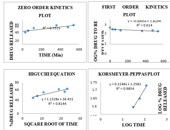
Figure 14 In vitro release Kinetics of Efinaconazole EF4 formulation
