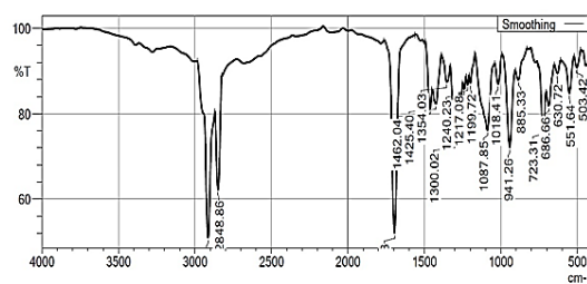
Figure 9 FTIR Spectrum of Efinaconazole SLN Formulation EF6
