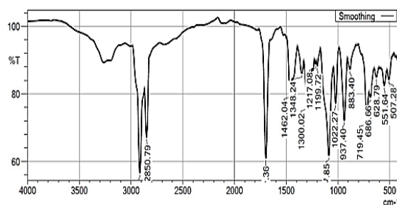
Figure 8 FTIR Spectrum of Efinaconazole SLN Formulation EF2
