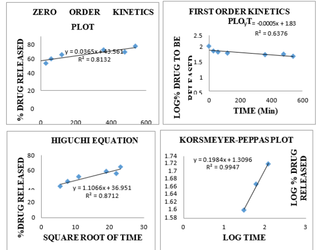
Figure 12 In-vitro release Kinetics of Efinaconazole selected EF2 Formulation
