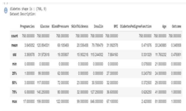
Figure 3: Dataset Description
