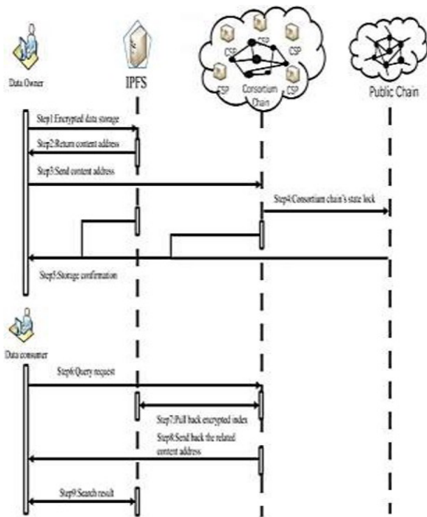
Fig.3. Ethereum based cloud security framework for SCM [8]
