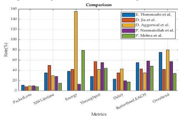
Fig. 4.: Comparison of different WSN parameters
