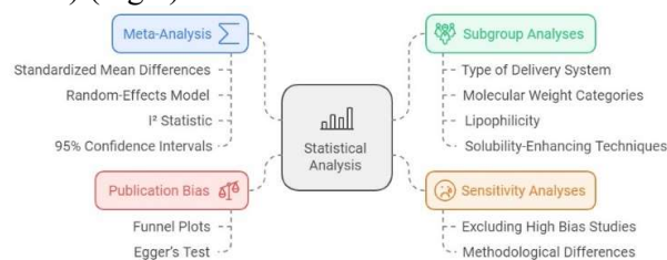
Fig.6. Statistical Analysis
