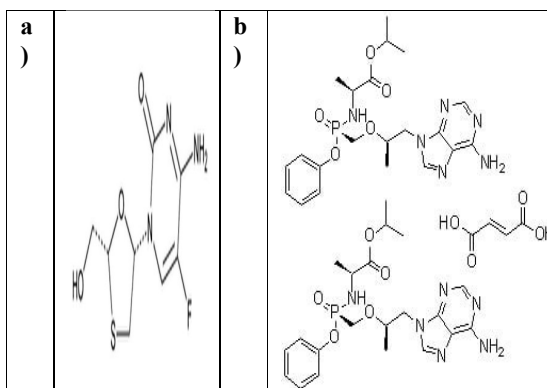
Figure 2: Chemical structures for a) Emtricitabine, b) Tenofovir Alafenamide Fumarate as Per USP
