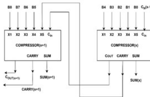
Figure 6 Approximate 5:2 compressor chain [22].
