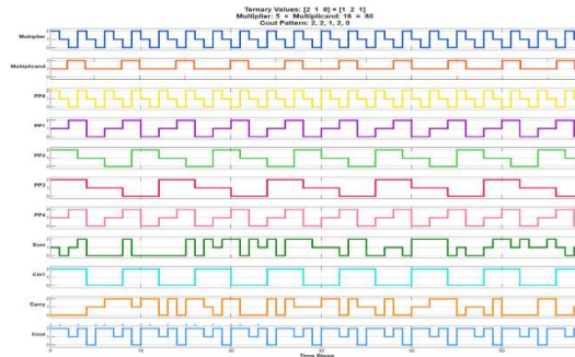
Figure 11 Simulation of input and output multiplicant with ternary logic based 5:2 compressors.
