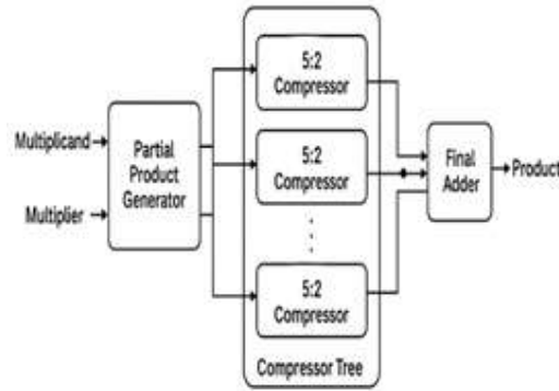
Figure 7 RTL design using 5:2 compressors with ternary logic gates [25].
