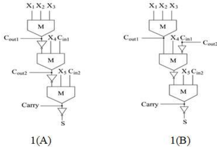
Figure 1 (A) MLAC-I and 1(B) MLAC-II diagrammatic representations of MLAC [7].
