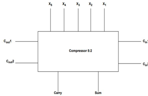
Figure 3 Block diagram of the 5:2 compressor [17]
