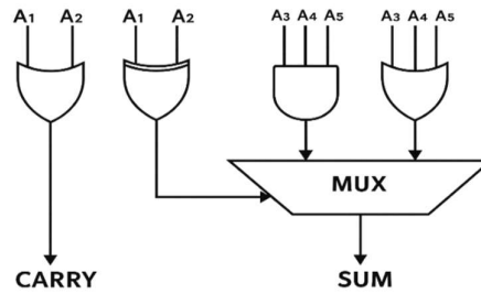
Figure 5 Approximate 5:2 compressor [20].
