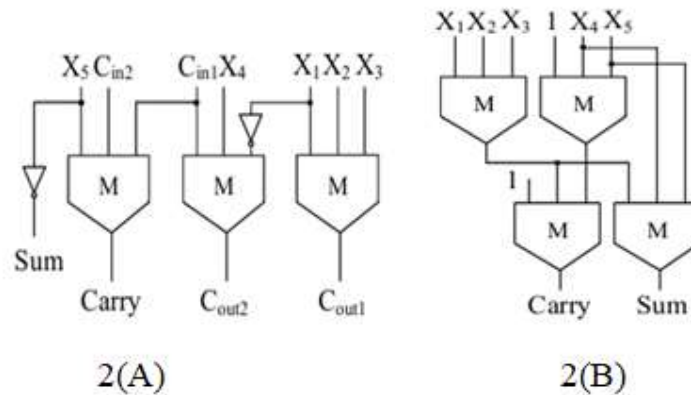
Figure 2 Displays the 5:2 MLAC as MLAC-III in 2(A) and MLAC-IV in 2(B) [7].
