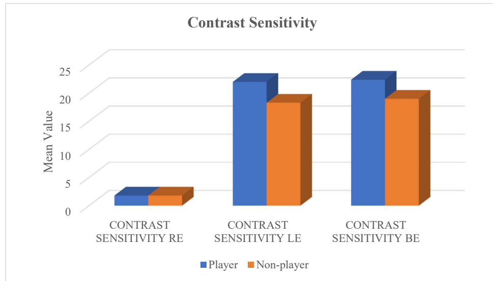
Figure 1. Contrast Sensitivity
