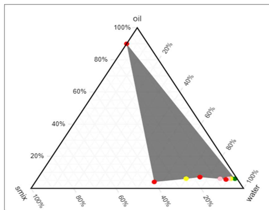
Figure 1: Ternary Phase Diagram for preparation of SMEDDS of Dasatinib
