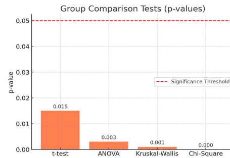
Figure 4: Group Comparisons (t-test, ANOVA, Kruskal-Wallis, Chi-Square)
