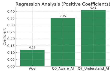
Figure 6: Regression Analysis
