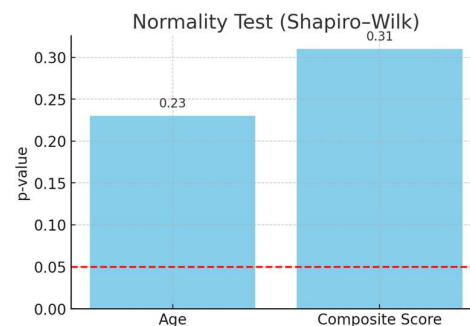
Figure 1: Normality Test (Shapiro-Wilk)
