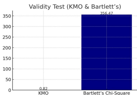
Figure 3: Validity Test (KMO & Bartlett's)
