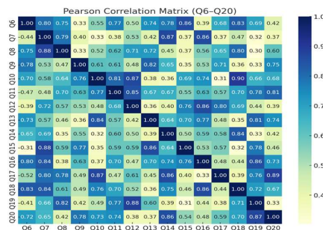
Figure 5: Pearson Correlation Matrix (Heatmap Figure)
