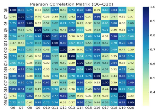
Figure 5: Pearson Correlation Matrix (Heatmap Figure)
