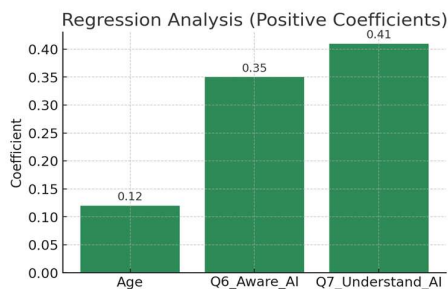
Figure 6: Regression Analysis
