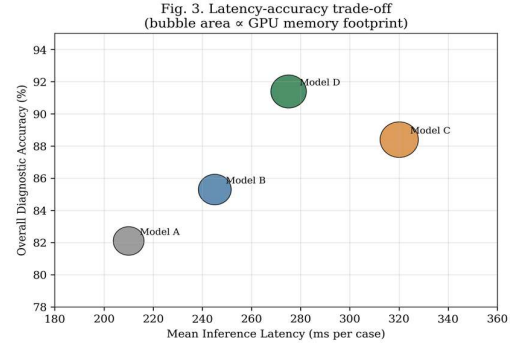
Fig. 3. Latency-accuracy trade-off across the four candidate architectures.
