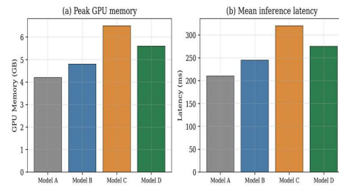
Fig. 4. Peak GPU memory (a) and mean inference latency (b) per case, by model.
