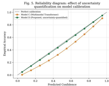
Fig. 5. Reliability diagram comparing Model C and the proposed uncertainty-quantified Model D.
