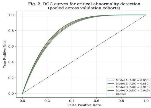
Fig. 2. Pooled ROC curves for critical-abnormality detection. AUC values are computed via Equation (6).
