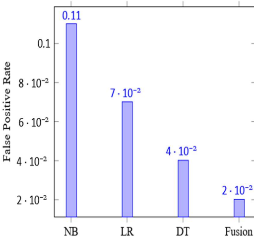
Figure 6 : False Positive Rate Comparison
