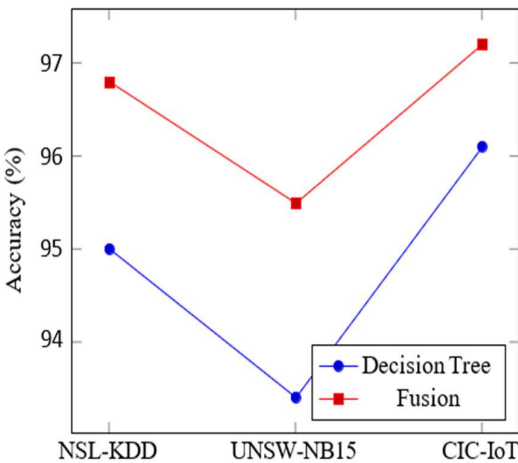
Figure 7 : Accuracy Comparison Across Datasets
