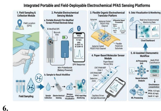
Figure 6. Portable and field-deployable electrochemical PFAS sensing platforms based on screen-printed electrodes, organic electrochemical transistors and paper-based molecularly imprinted polymer devices for rapid in situ monitoring. Also illustrated are smartphone-assisted analytics, wireless data transmission and AI-enabled chemometric interpretation for multiplex PFAS analysis.
