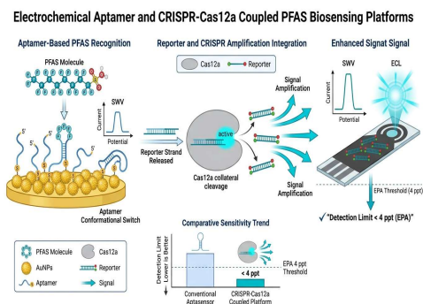
Figure 5. Electrochemical biosensing architectures involving aptamer-based recognition, and CRISPR-Cas12a amplification approaches, for ultrasensitive detection of PFAS. The figure also compares the signal amplification efficiency with the detection limits with respect to the EPA 4 ppt regulatory threshold.
