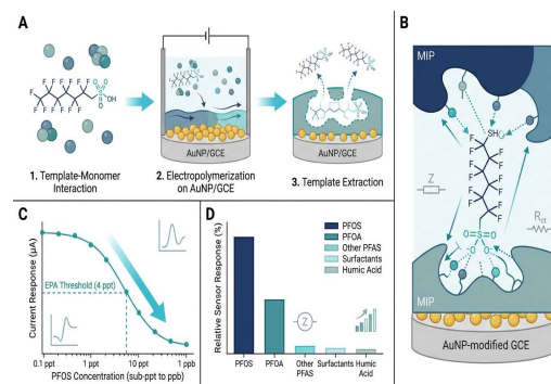
Figure 4. Schematic representation of molecularly imprinted polymer preparation, selective PFAS recognition, and electrochemical sensing performance on AuNP/GCE platforms. The calibration behaviour and selectivity towards PFOS over structurally related interferences are also shown.
