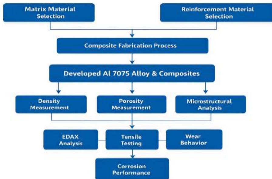
Figure 3.1 illustrates the flowchart of the experimental procedure adopted for the present investigation. The study includes the selection of matrix and reinforcement materials, identification of the composite fabrication process, and characterization of the developed Al 7075 alloy (AST0) and its composites. Detailed investigations were carried out on density, porosity, microstructural features, EDAX analysis, tensile properties, wear behavior, and corrosion performance.
