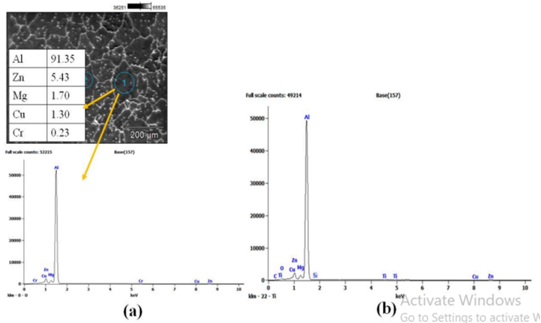
Figure 4.6 EDAX of (a) AST0 and (b) AST15
