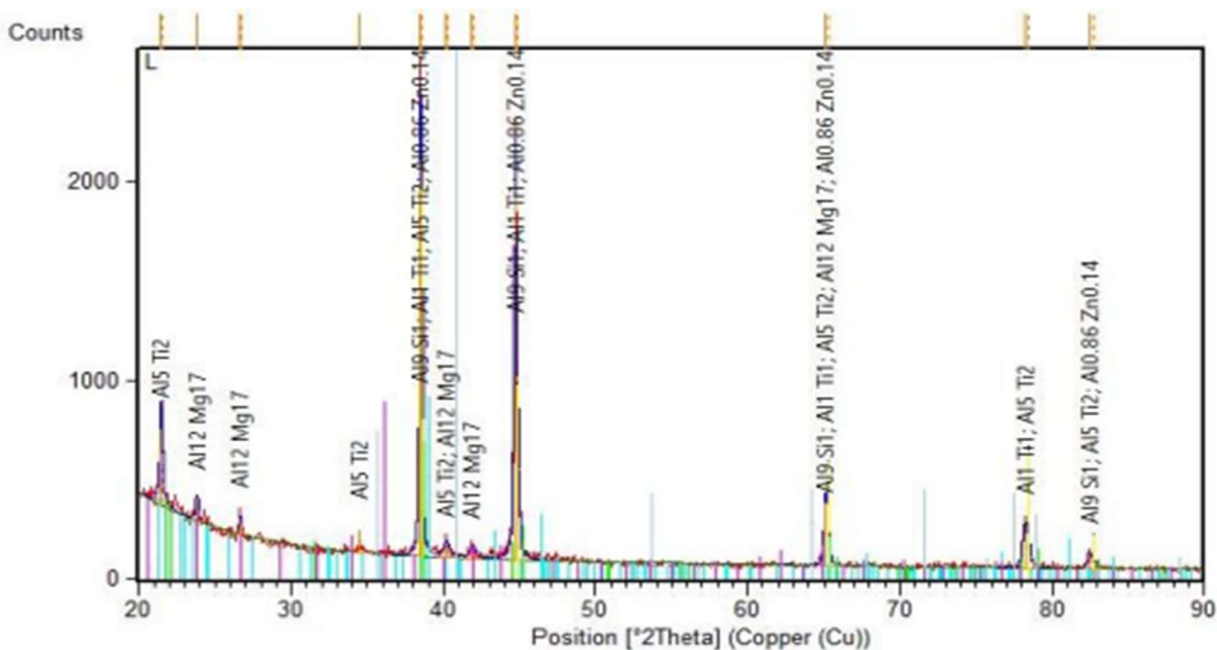
Figure 4.2 Intermetallic peaks identified
