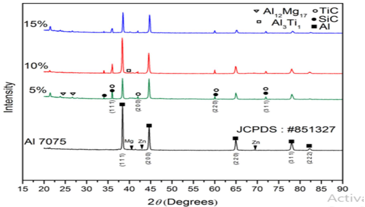
Figure 4.3 XRD image of SiC and TiC reinforced aluminium 7075 composites
