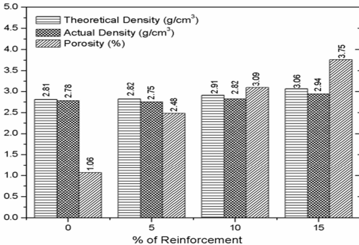
Figure 4.1 Densities and porosity of Al 7075 composites
