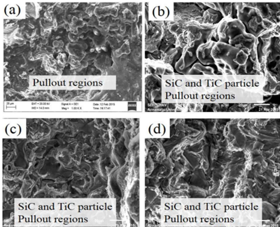
Figure 4.7 SEM micrographs of tensile fracture surface (a) AST0, (b) AST5, (c) AST10 and (d) AST 15
