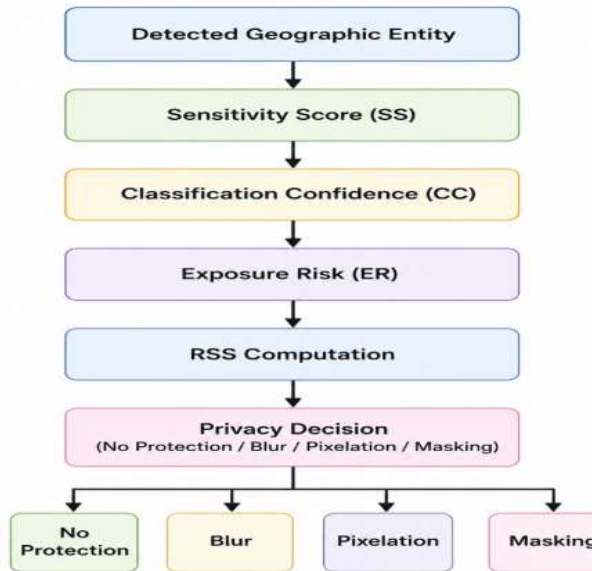
Figure 2: Workflow for Relative Sensitivity Score (RSS) Computation
