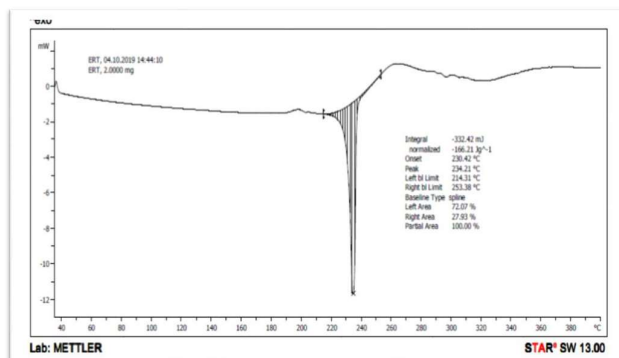
Figure 7 : DSC of Azathioprine
