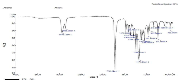
Figure 6: FTIR range of drug and polymer
