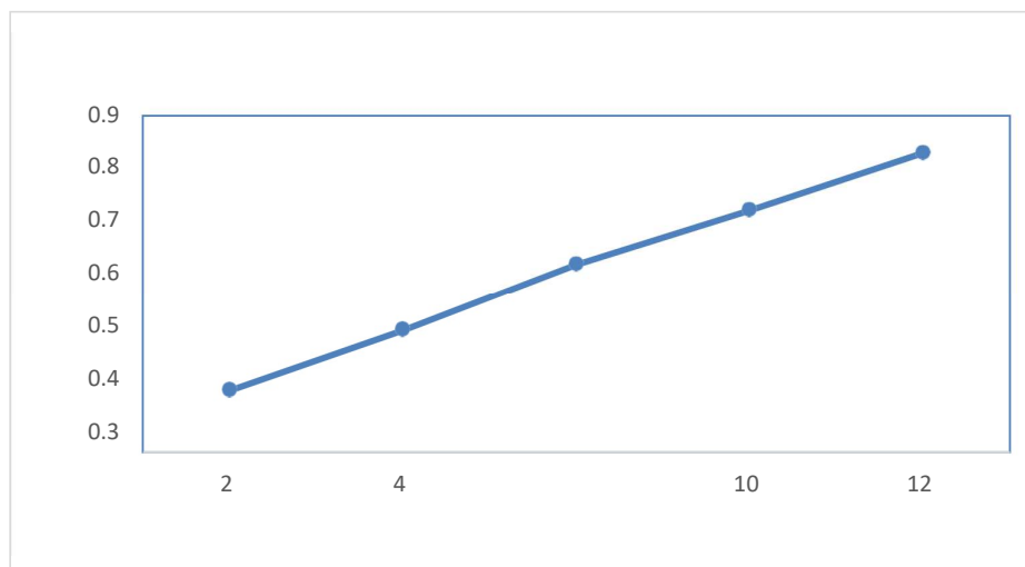
Figure 5: Calibration of Azathioprine
