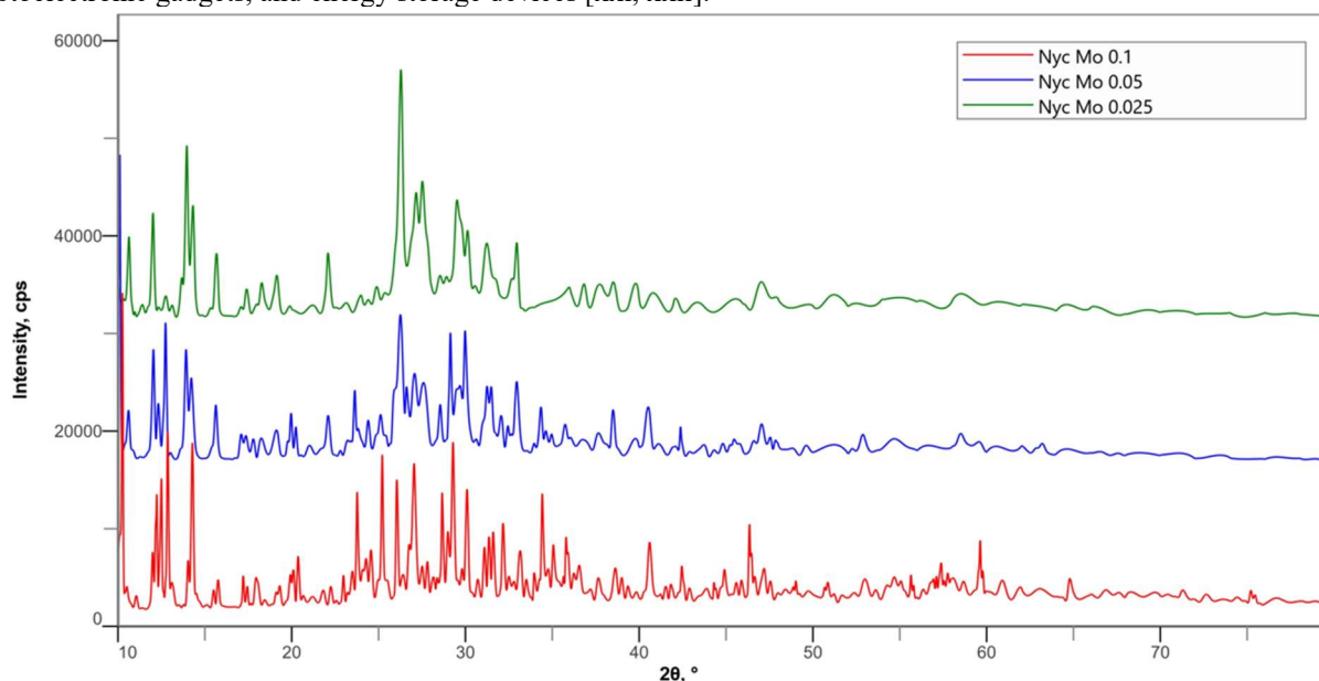
Fig. 2: X-Ray Diffraction analysis of MoO 3 Nanoparticles under varying extract concentrations
