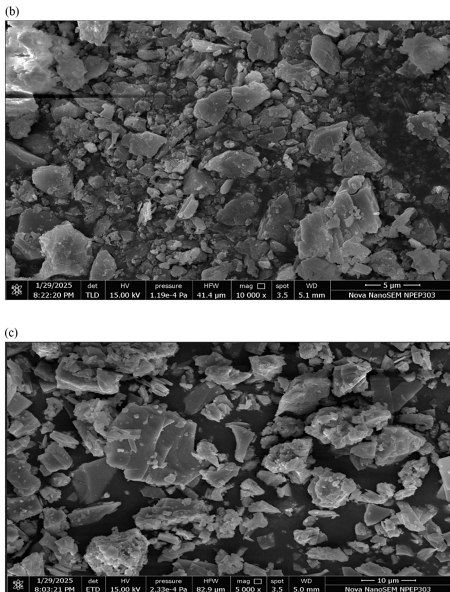
Fig. 3: FESEM of Nyctanthes -mediated \text{MoO}_3 Nanoparticles under varying extract concentrations (a) 0.025M, (b) 0.05M, and (c) 0.1M
