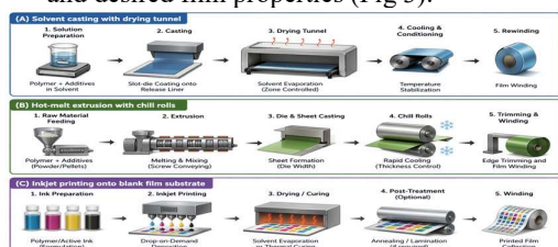
Figure 3 : Process flow diagram comparing manufacturing technologies: (A) Solvent casting with drying tunnel, (B) Hot-melt extrusion with chill rolls, (C) Inkjet printing onto blank film substrate. Include key process parameters for each method.
