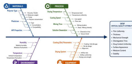
Figure 5: Ishikawa (fishbone) diagram illustrating factors affecting OFDF critical quality attributes. Include branches for Materials, Process, casting speed, Environment, and Equipment
