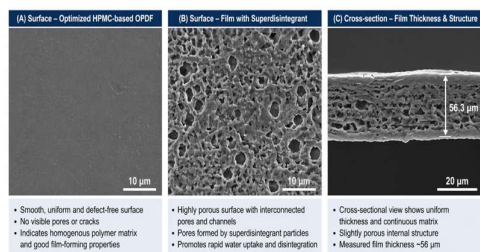
Figure 4: SEM Images of Oro dispersible Films Showing Surface and Cross-Sectional Morphology.
