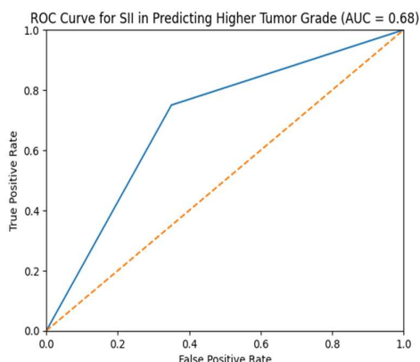
FIGURE:1 ROC curve for SII in predicting higher tumor grade. It visually represents the diagnostic performance of SII as a prognostic marker.
