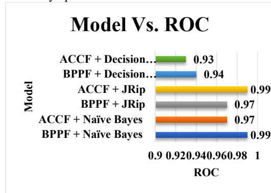
Figure 5: Model Vs ROC
