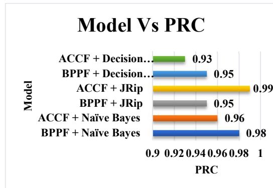
Figure 6: Model Vs PRC
