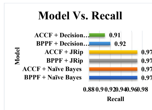
Figure 4: Model Vs Recall
