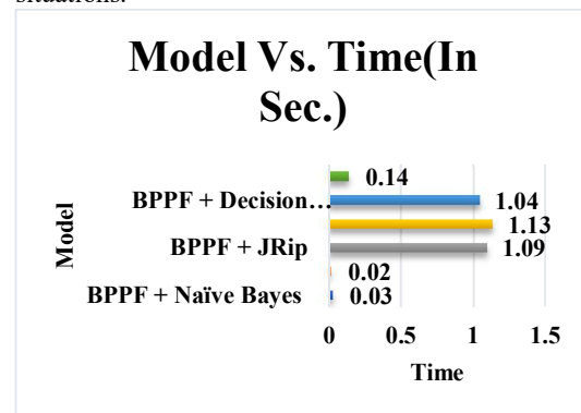
Figure 7: Model Vs Time (In Sec.)
