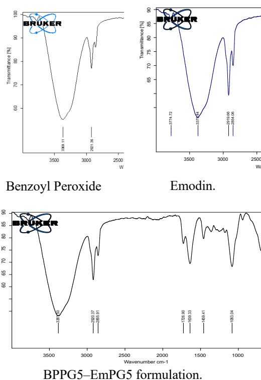
Figure 1. FTIR spectra of Benzoyl Peroxide, Emodin, and the optimized BPPG5–EmPG5 formulation.
