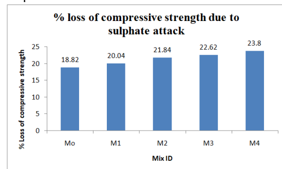
Graph 10: Comparison of percentage loss of strength
