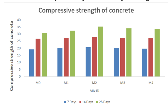
Graph 3: Comparison of Compressive strength
