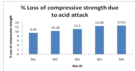
Graph 7: Comparison of percentage loss of strength
