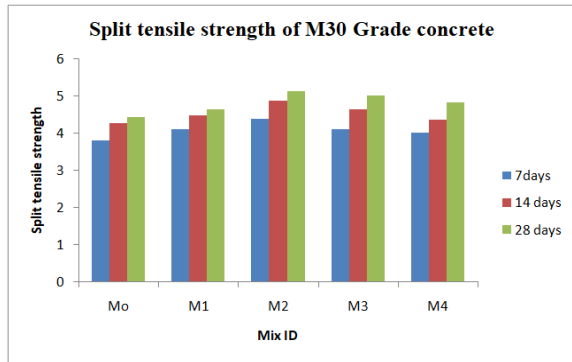
Graph 4: Comparison of Tensile strength
