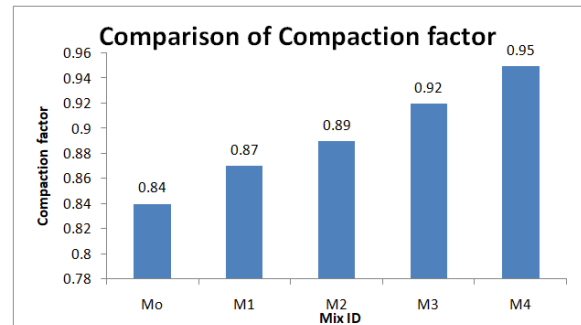
Graph 2: Comparison of compaction factor
