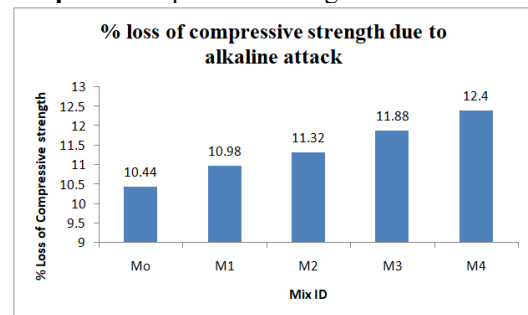
Graph 9: Comparison of percentage loss of strength
