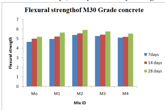
Graph 5: Comparison of Flexural strength
