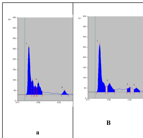
Figure 3: [a] HPTLC chromatogram of MEF1 extract measured at 366nm [b] HPTLC chromatogram of CEF3 extract measured at 366nm
