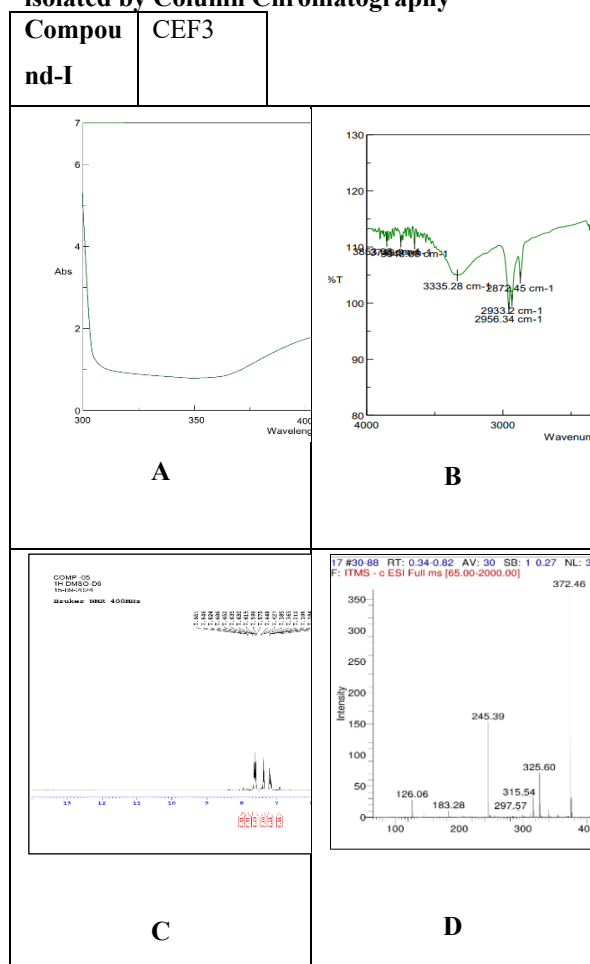
Figure:5 [a] UV graph of Compound – I [b] IR spectra of compound-I [c] Proton NMR spectrum of Compound –I [d] MASS spectrum of Compound –I
