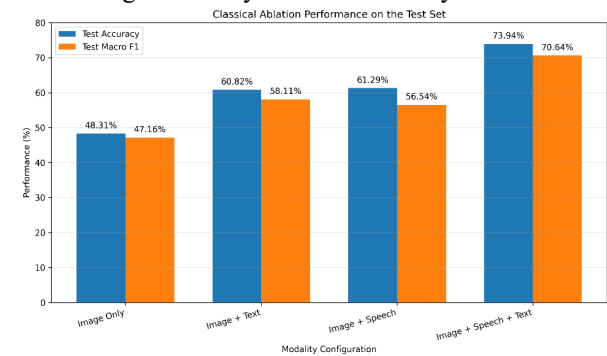
Figure 4. Classical ablation performance across different modality configurations on the held-out test set.
