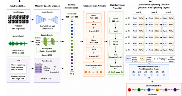
Figure 1. Overall architecture of the proposed hybrid quantum–classical framework for six-class multimodal emotion recognition. Facial images from FER-2013, speech from VED, and text data are processed by modality-specific encoders to obtain 512-, 128-, and 128-dimensional representations, respectively. The representations are concatenated and transformed through classical fusion to a 128-dimensional
