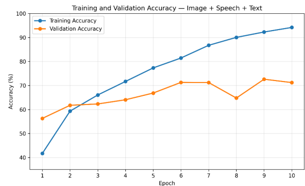
Figure 3. Training and validation accuracy of the Image + Speech + Text multimodal model over 10 epochs.
