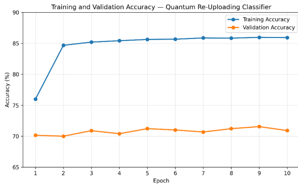
Figure 7. Training and validation accuracy of the quantum re-uploading classifier over 10 epochs.
