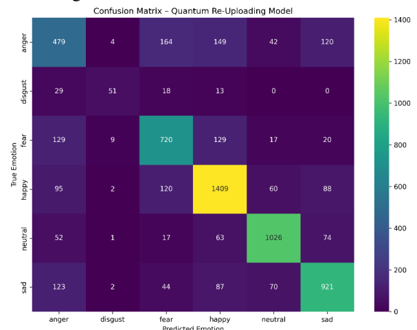
Figure 8. Confusion matrix of the quantum re-uploading classifier on the held-out test set.
