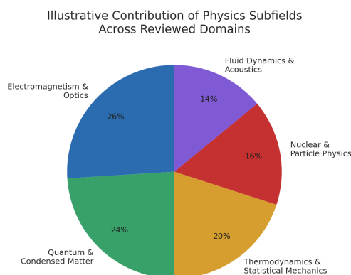
Figure 3. Illustrative contribution of major physics subfields across the domains reviewed in this paper.
