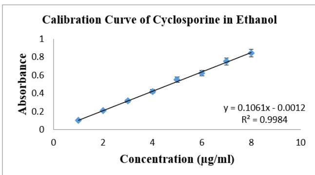
Figure 1.9: Calibration curve of Cyclosporine in Ethanol
